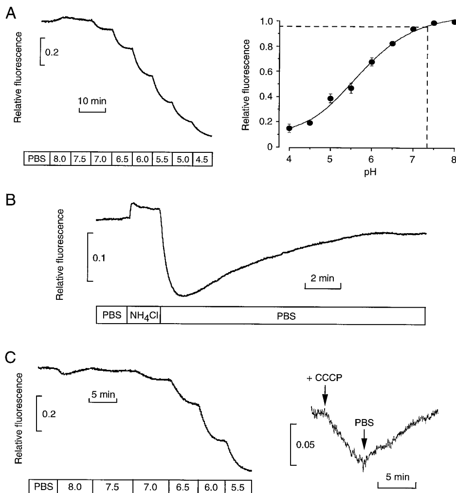
FIGURE 5 GFP as an intracellular pH indicator. (A) Titration of fluorescence versus pH in LLC-PK1 cells expressing GFP-F64L/S65T. Cells were initially perfused with PBS and then with buffer B containing ionophores at indicated pH (see Materials and Methods); (left) Representative titration curve; (right) Averaged fluorescence (SE, n = 4 ) with fit to Eq. 1. (B) Time course of cytoplasmic GFP-F64L/S65T fluorescence in response to replacement of 30 mM NaCl by \text{NH}_4\text{Cl} and subsequent return to NaCl. (C, left) Titration as in A for CHO cells expressing GFP-F64L/S65T in mitochondria; (right) Response of mitochondrial GFP-F64L/S65T fluorescence to addition of the protonophore CCCP (10 \mu\text{M} ) to the PBS perfusate.
